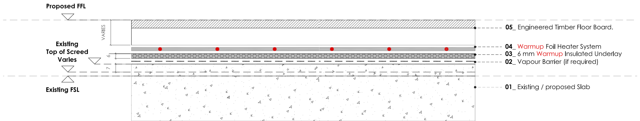
WARMUP UNDERFLOOR HEATING FOIL HEATER SYSTEM ( WOOD )
